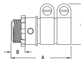
Sizes 2-1/2" - 4" are manufactured as shown above.
