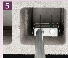
Top view: EMT installed in box.
