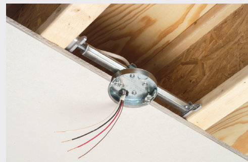
Cut away showing FBR5407R installed between wood I-beams
