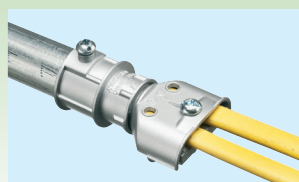
3/4" EMT to 2410 to 846 with NM cable
