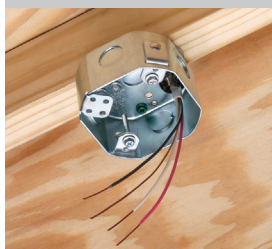
FBS415/FBS420 Mount UNDER Joist
