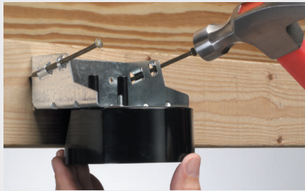
Nails to the joist for a super secure installation! All photos shown with FB417S
