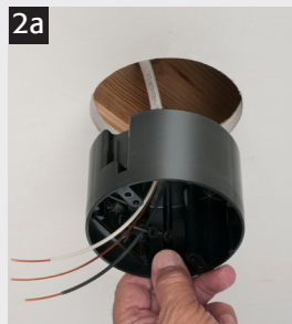
2a ...through installed NM942 cable connector. Insert box into opening.
