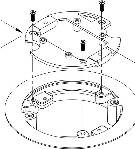
FLBC4520 Installation on FLBC4800 Concrete Can
