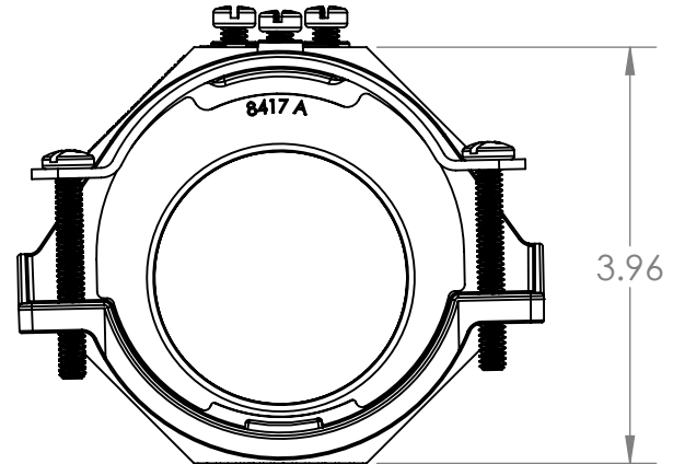
AI CAT#841717 3" SET SCREW TO 3" MC TRANSITION FITTING
