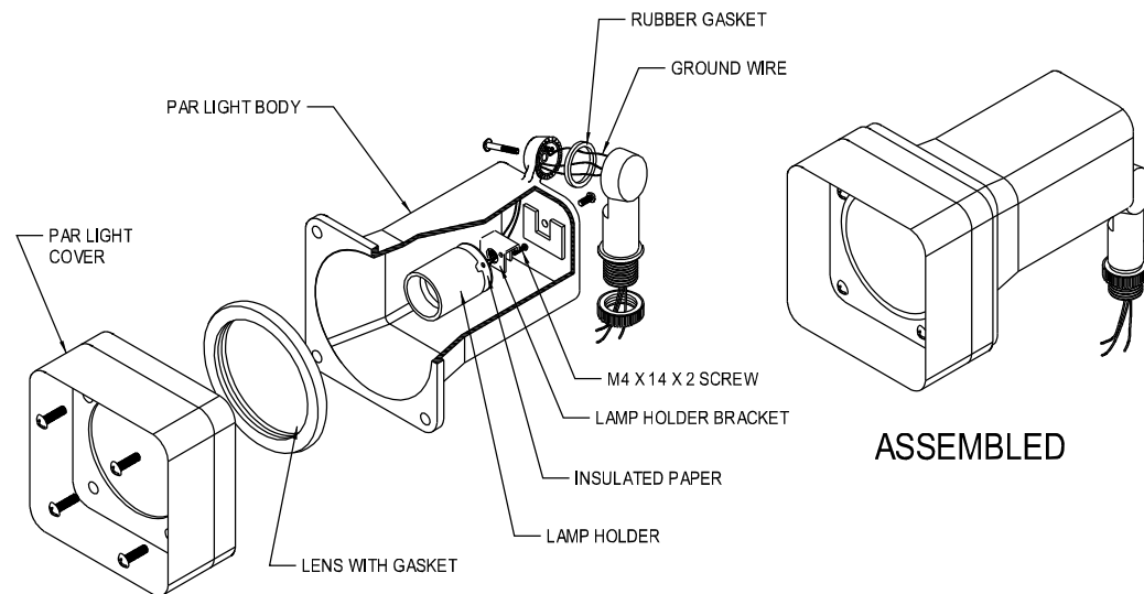
ISOMETRIC ASSEMBLY VIEW
