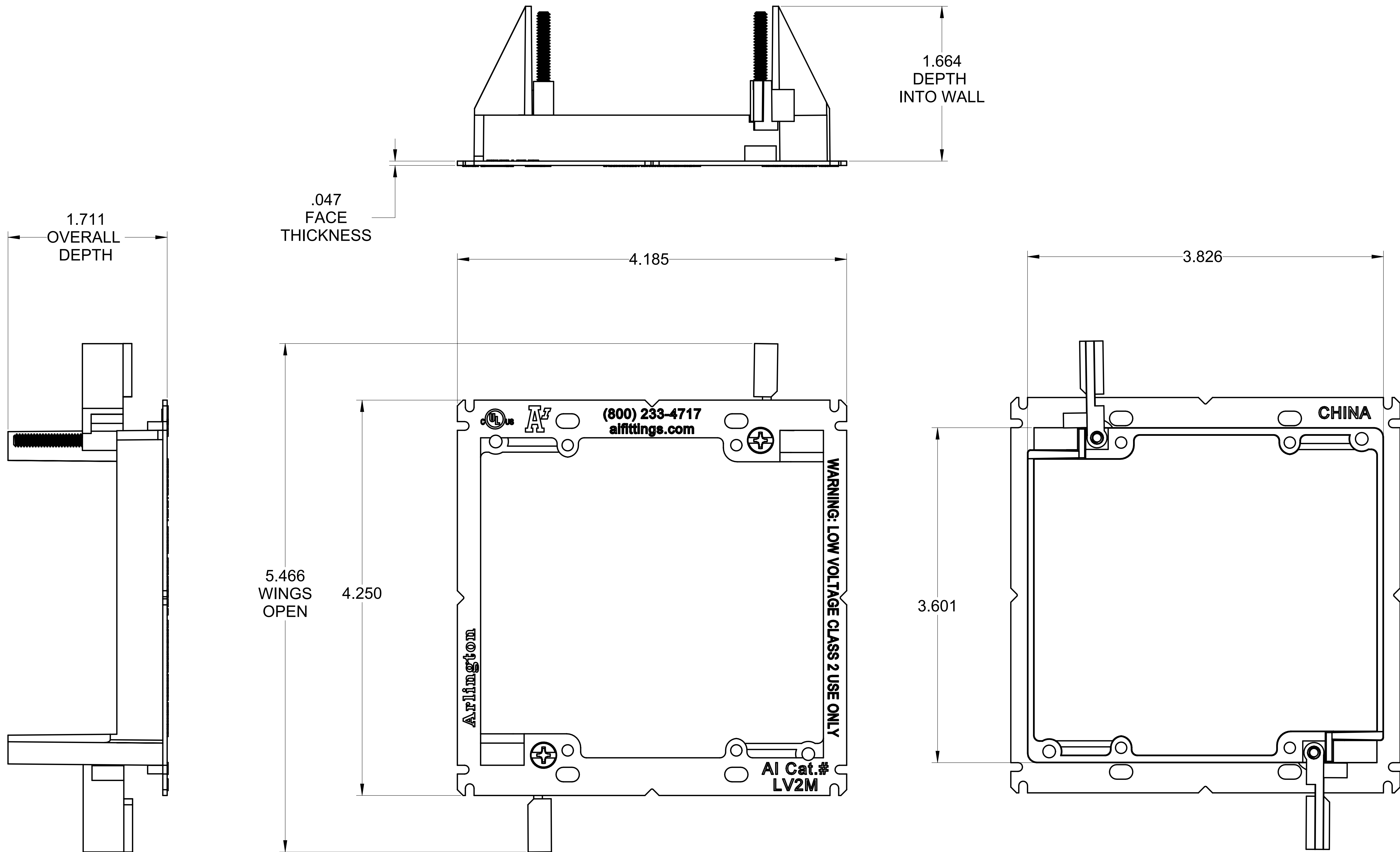
REAR VIEW (INTO WALL)
