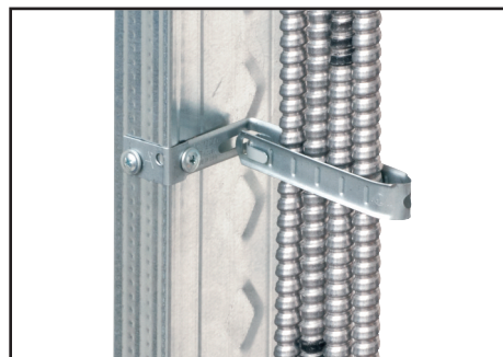
4 Bend tab over support to lock cable securely in place. CUS6 holds up to FOUR MC cables – or SIX NM Cables centered on a 2x4.
