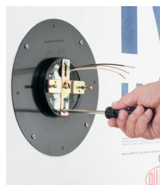
Install fixture mounting hardware per fixture manufacturer's instructions.
