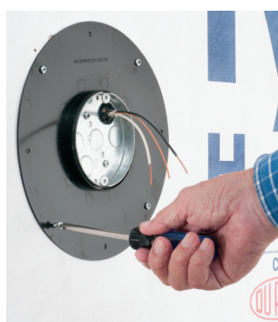
Attach flashing backing to sheathing through flashed-over holes.
