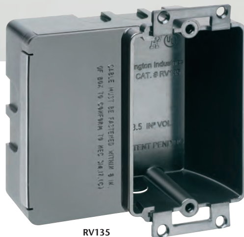
RV135 Shallow depth single-gang device box
